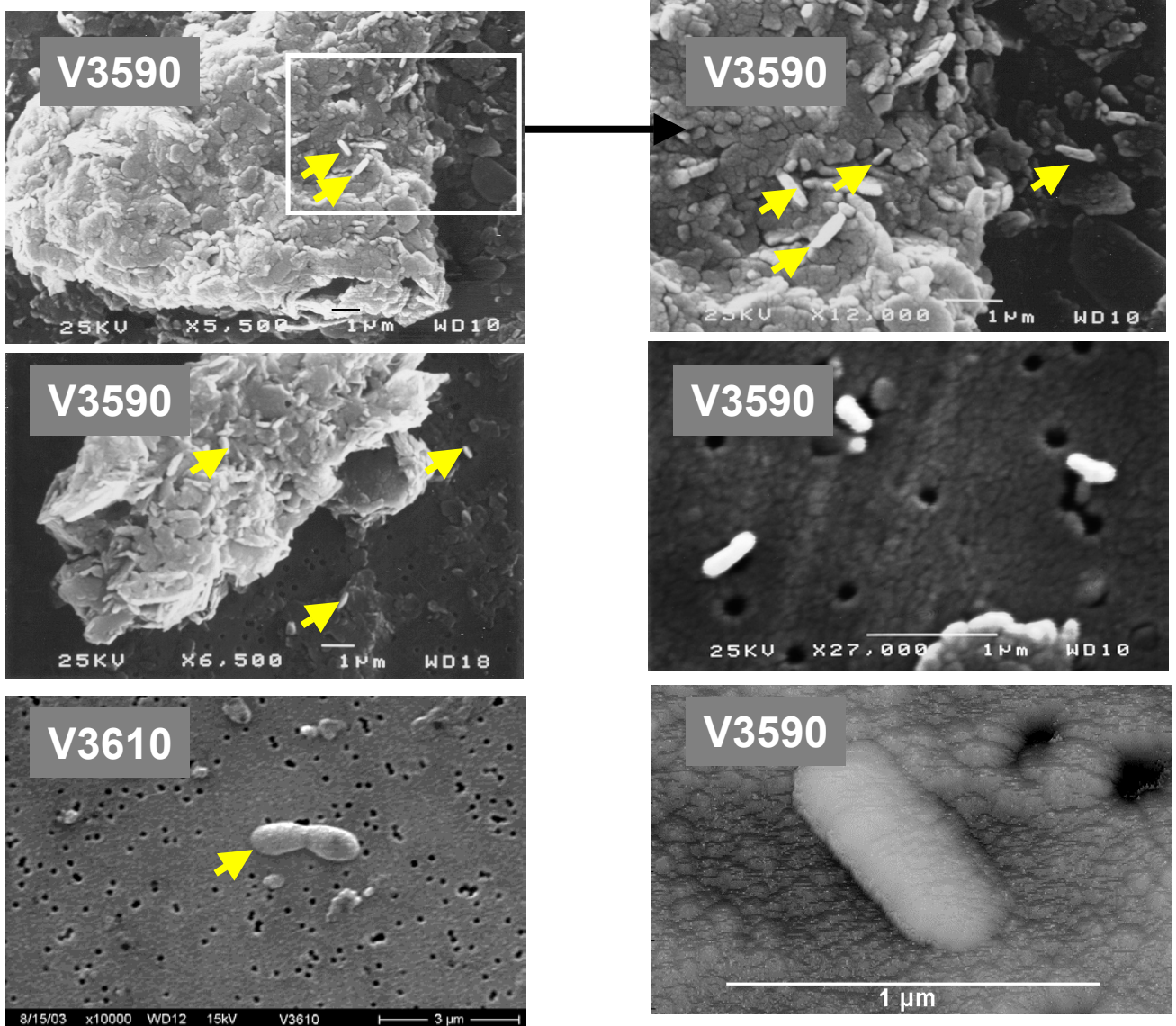
Figure 2. Scanning electron micrographs of microbes in Lake Vostok accretion ice. Samples are designated by their depth of recovery from below the surface in meters and yellow arrows indicate prokaryotic cells. Melt water was filtered onto 0.2µm polycarbonate filters sputter coated with 10 nm Au-Pd and imaged using a cryogenic scanning electron microscope. Adapted from Priscu et al. 1999, Science , 286:2141-2144.
